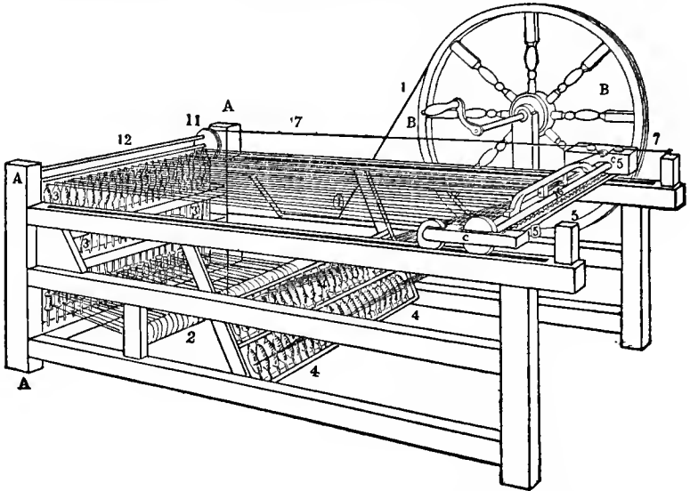
FIG. 3. IMPROVED MODEL OF HARGREAVES'S SPINNING JENNY
